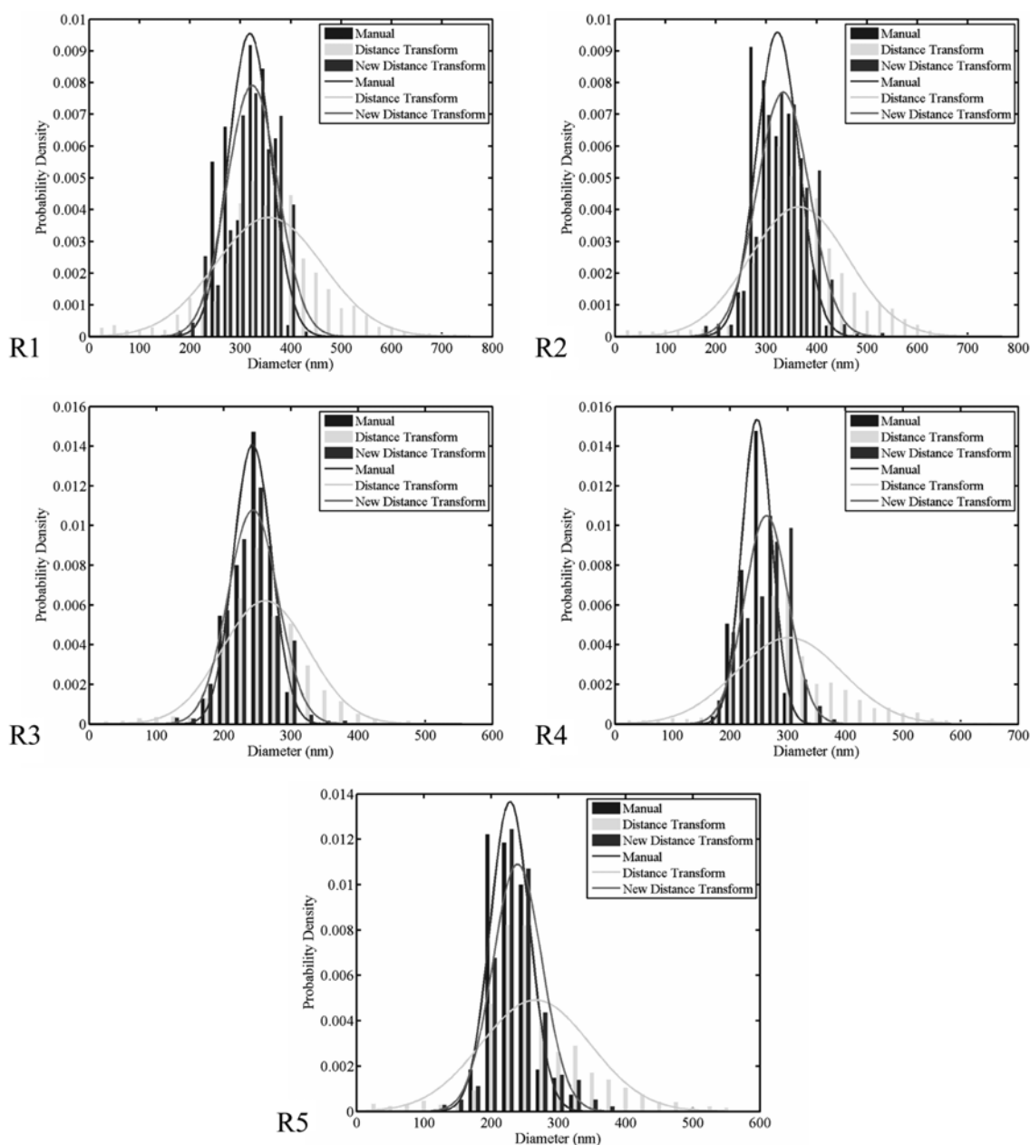
Fig. 19. Histograms for real webs.
