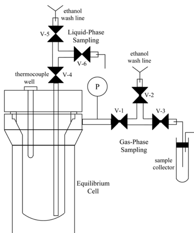
Fig. 1. The equilibrium cell and sampling lines.
