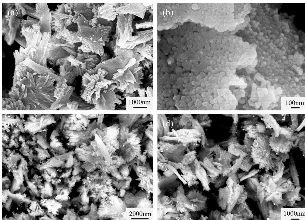
Fig. 2. SEM images of ZnO (a and b), Ag/ZnO-1 (c) and Ag/ZnO-2 (d).
