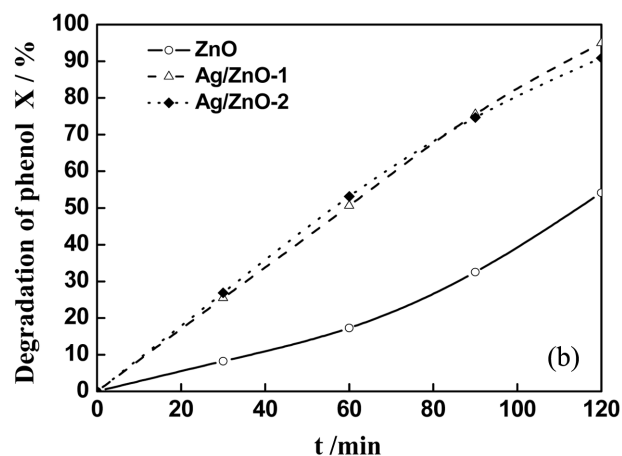
Fig. 5. Photocatalytic activity of ZnO and Ag/ZnO for degradation of methyl orange (a) and phenol (b).
