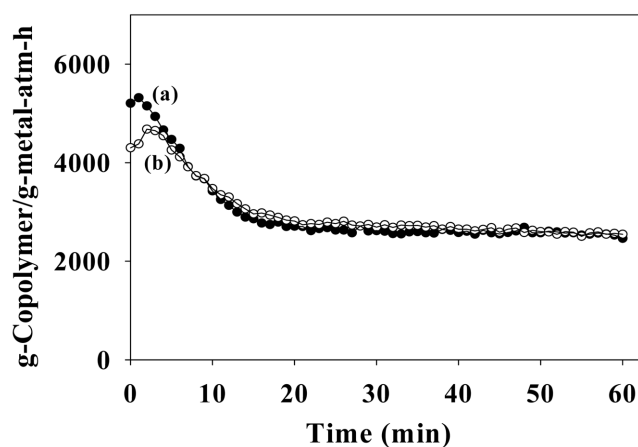
Fig. 2. Activity profiles of rac - \text{Et}(\text{Ind})_2\text{ZrCl}_2/\text{TiCl}_4/\text{MAO/SMB} catalyst in the ethylene-hexene copolymerization with a variation of cocatalyst species: (a) TIBAL and MAO, (b) TEA and MAO.
