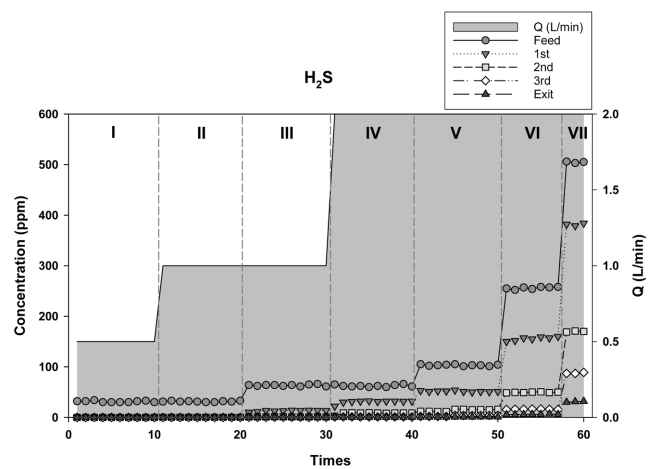
Fig. 2. Various hydrogen sulfide concentrations of biofilter process at each sampling port (1st, 2nd, 3rd and exit) versus experimental times.
