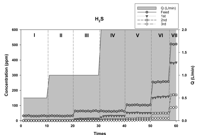
Fig. 3. Various hydrogen sulfide concentrations of biofilter process at feed inlet, 1st, 2nd and 3rd sampling ports.
