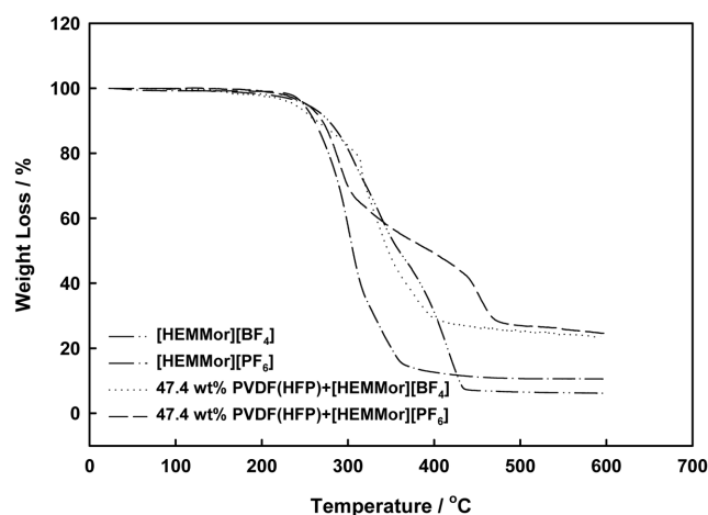
Fig. 6. TGA data of neat ionic liquids and of 47.4 wt% PVdF(HFP)-ionic liquid gels based on [HEMMor][BF 4 ] and [HEMMor][PF 6 ].
