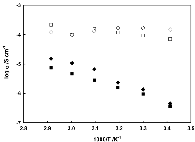
Fig. 11. Ionic conductivity of the PVdF(HFP) gel in [HEMMor][PF 6 ] system as a function of temperature: 0 wt% PVdF(HFP) (■), 33.3 wt% PVdF(HFP) (◆), 47.4 wt% PVdF(HFP) (◇), 66.7 wt% PVdF(HFP) (□).
