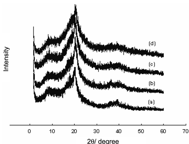
Fig. 8. XRD patterns of PVdF(HFP)-[HEMMor][BF 4 ] gels: (a) 100 wt% PVdF(HFP), (b) 66.7 wt% PVdF(HFP), (c) 47.4 wt% PVdF(HFP), and (d) 33.3 wt% PVdF(HFP).
