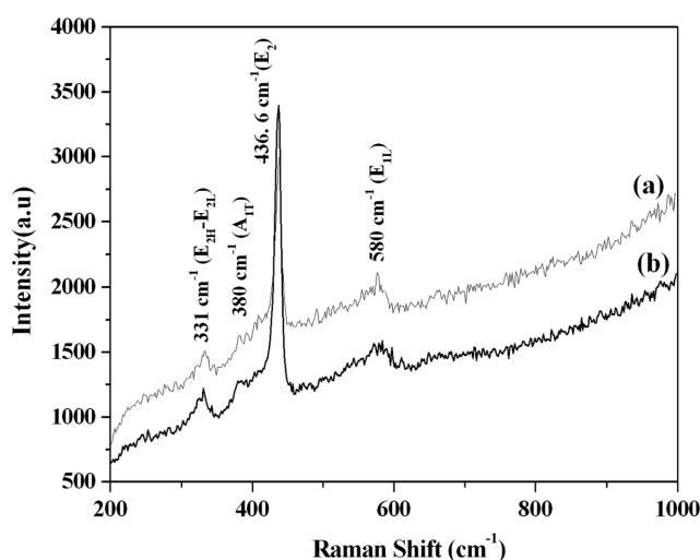
Fig. 5. Raman spectra for the ZnO nanowires grown on steel alloy substrates: (a) as-grown and (b) after annealing at 450 °C in an oxygen atmosphere for 15 min.
