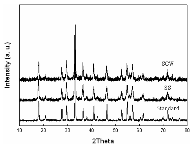
Fig. 5. XRD patterns of synthesized YAG : Eu phosphor at SCW (Conc.=Eu 10 at%, pH=9.41) and solid-state methods.
