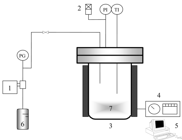
Fig. 1. Schematic diagram of experimental batch SCW apparatus.
