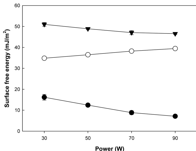
Fig. 2. Surface free energy with respect to power ( \blacktriangledown total, \circ dispersion, \bullet polar).
