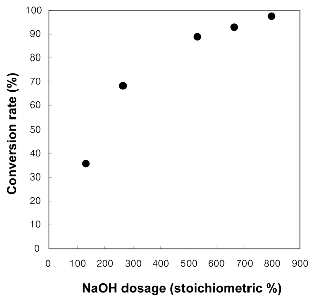
Fig. 7. Conversion variation of 2,4-DCP with NaOH pre-dosage and without H_2O_2 at 1,000 mg/L of 2,4-DCP, 250 bar and 400 °C.
