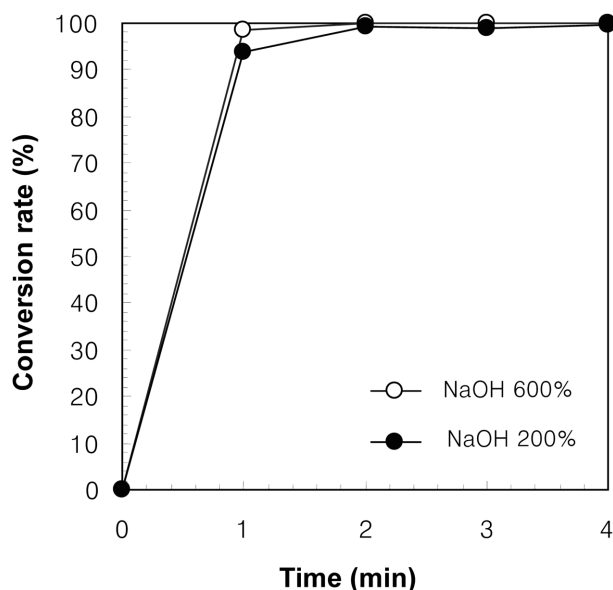
Fig. 8. Conversion variation with residence time at pre-dosage of NaOH and 400% H_2O_2 .
