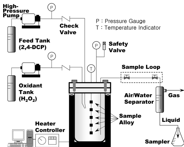
Fig. 1. Schematic diagram of SCWO process.
