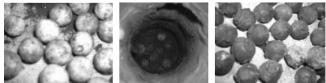
Fig. 8. Clogged pebble bed caused by the oversupplied coal.
