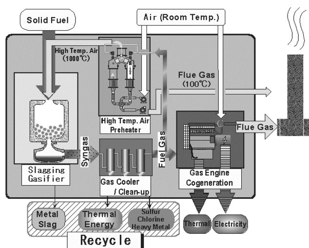
Fig. 1. Syngas production and utilization system by MEET method.
