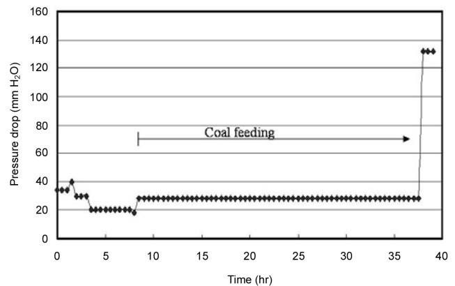
Fig. 7. Pressure drop measured at pebble bed.
