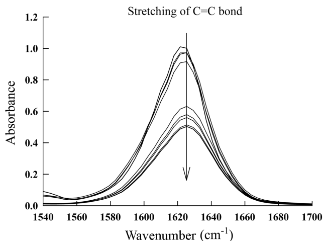
Fig. 3. Typical decay of the stretching vibration bands of dimethacrylate double bonds at 1,638 \text{cm}^{-1} (time interval=0.2 sec).
