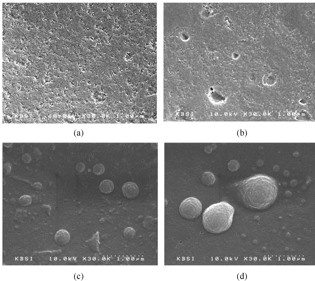
Fig. 6. SEM images photopolymerized TPU/acrylate blends (0 phr (a), 20 phr (b), 30 phr (c), and 40 phr (d) of TPU).
