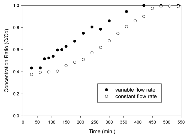
Fig. 10. The effect of one peak in flow rate on chloride breakthrough curve.
