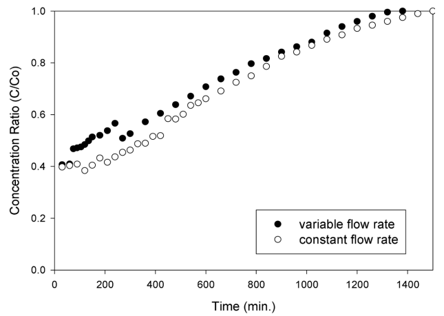
Fig. 9. The effect of one peak in flow rate on sodium breakthrough curve.
