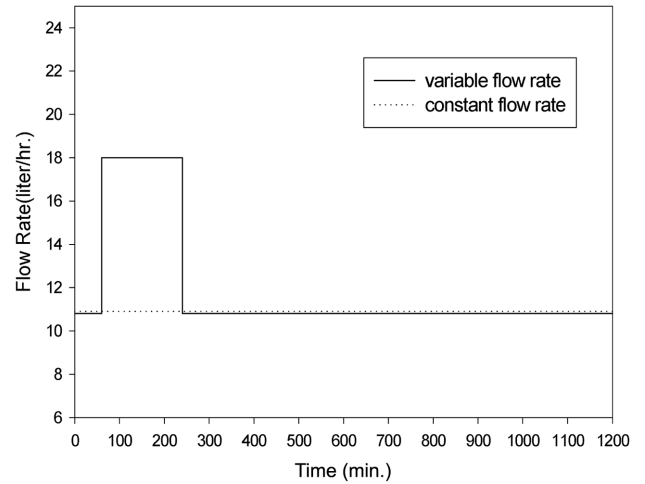
Fig. 8. Flow rate profiles for constant and variable flow rate experiments with one peak.
