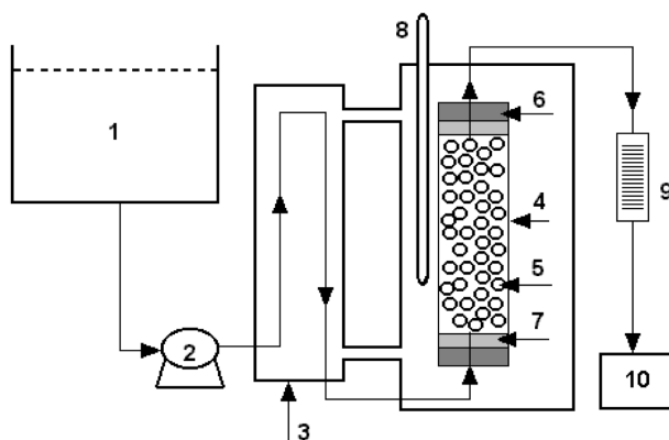
Fig. 1. Schematic diagram of the continuous column system.
