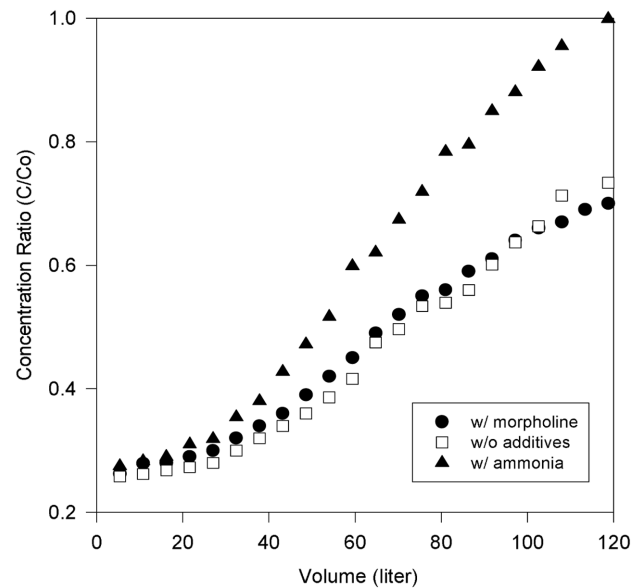
Fig. 5. The effects of amine additives on breakthrough curve of sodium with FCR=2 : 1 at 30 °C.
