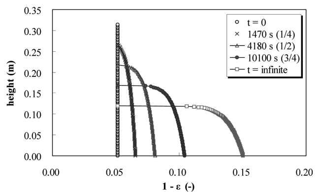
Fig. 9. The porosity and sedimentation height during sedimentation of the 12.9 wt% CaCO 3 suspension.
