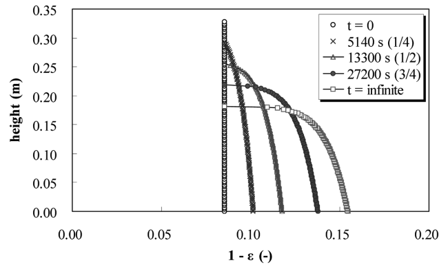
Fig. 8. The porosity and sedimentation height during sedimentation of the 20.9 wt% CaCO 3 suspension.
