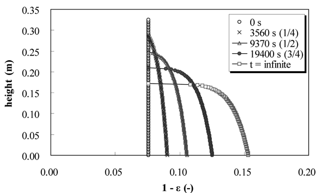
Fig. 7. The porosity and sedimentation height during sedimentation of the 18.6 wt% CaCO 3 suspension.
