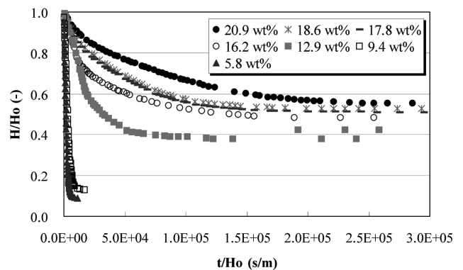
Fig. 3. Experimental results of hindered sedimentation from 5.8 to 20.9 wt% \text{CaCO}_3 suspension.
