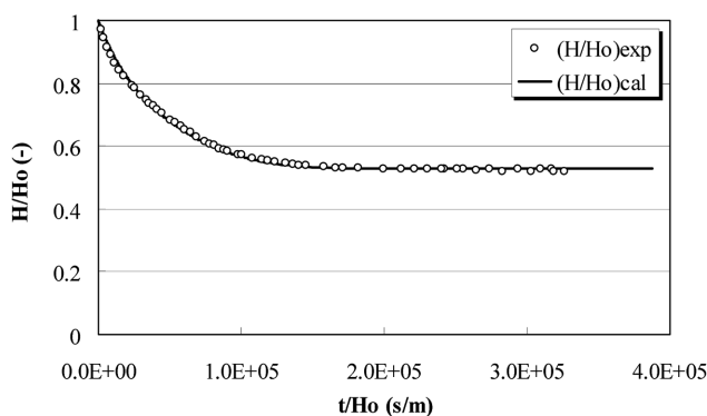
Fig. 4. Experimental and calculated results of hindered sedimentation for the 18.6 wt% CaCO 3 suspension.
