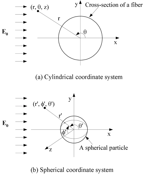
Fig. 1. Coordinate systems of (r, \theta, z) and (r', \phi', \theta') used in this study.
