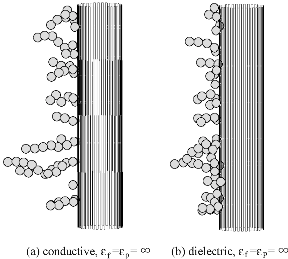
Fig. 9. Comparison of particle deposition patterns between the conductive and dielectric particles and fibers at E_0 = 15 kV/cm, U_0 = 5 cm/s. \varepsilon_f and \varepsilon_p are the dielectric constants of fiber and particle, respectively.
