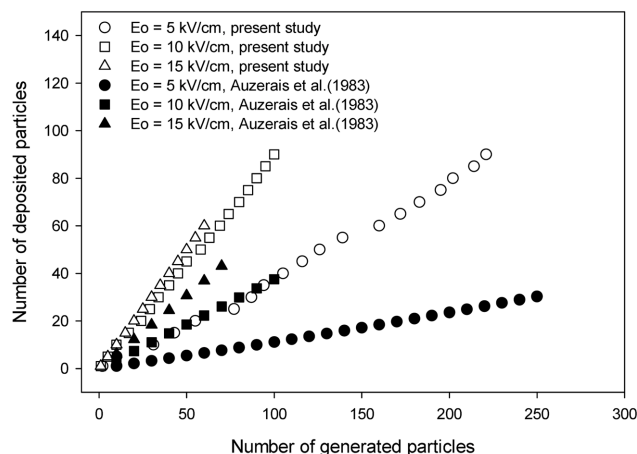
Fig. 12. Comparison of deposition rates in this study with those of Auzerais et al. [1983] for various electric field strengths at U_0 = 5 cm/s.
