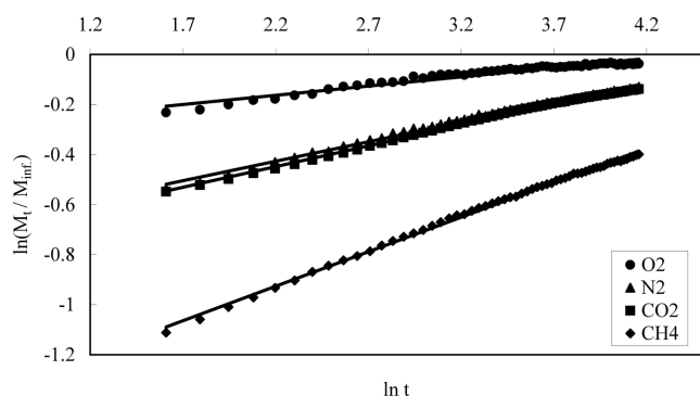
Fig. 5. Diffusivity of various gases on CCMg60. -\ln(M_t/M_{inf}) versus \ln t .
