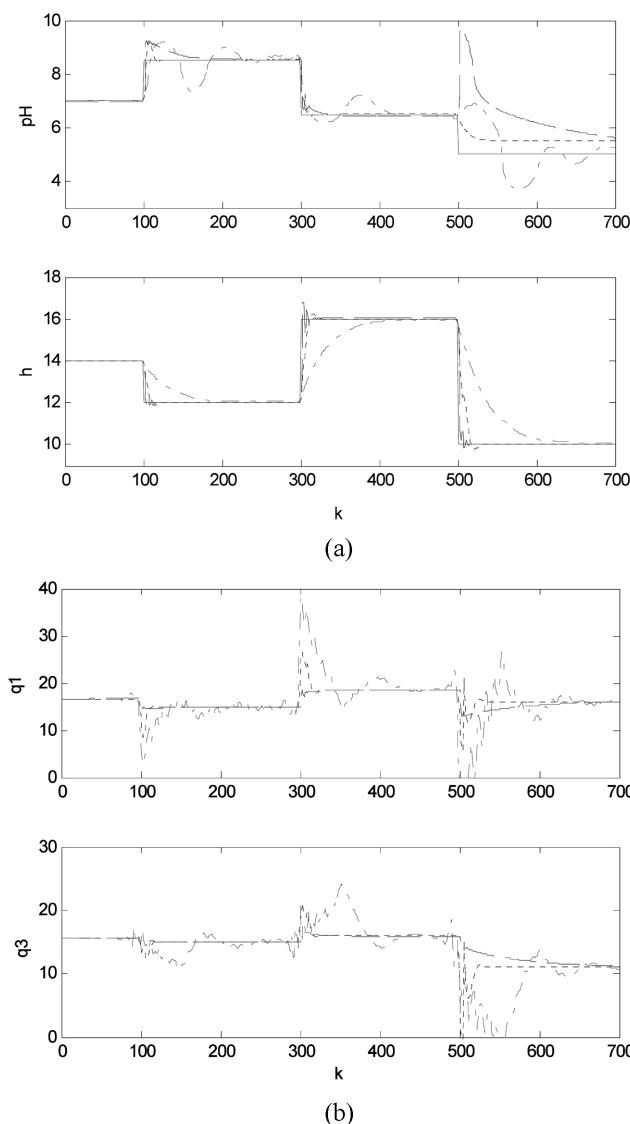
Fig. 10. Control performance of the setpoint changes (solid line) based on QDMC (dashdot line), NNMPC (dotted line) and proposed model (dashed line) in Example 2: (a) and h ; (b) q_1 and q_3 .
