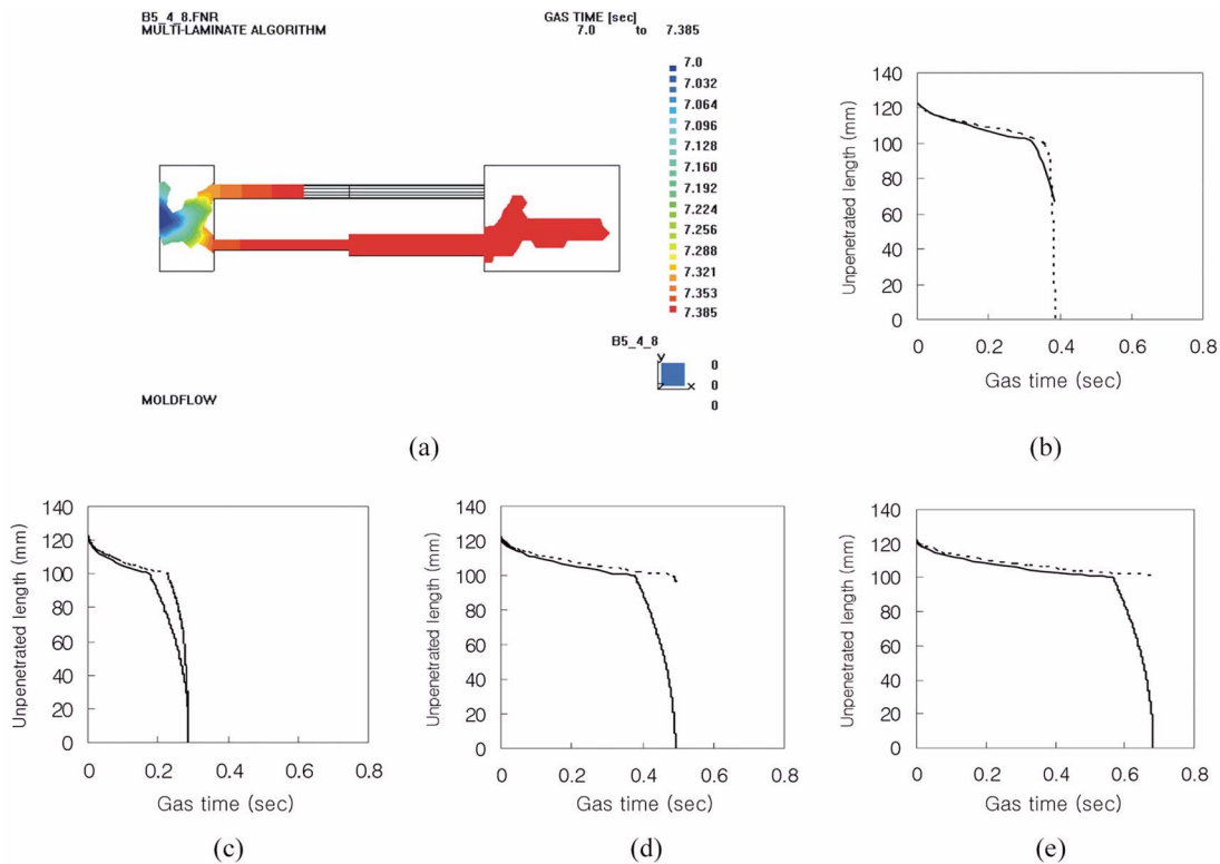
Fig. 7. (a) The geometry is the same as Fig. 6 except that diameter of pipe 21 is 4 mm; (b) Time evolution of gas penetration length from Fig. 7(a); Model predictions; (c) \theta = 0.93 ; (d) \theta = 2/3\pi ; (e) \theta = \pi (solid line: upper side, dotted line: lower side).
