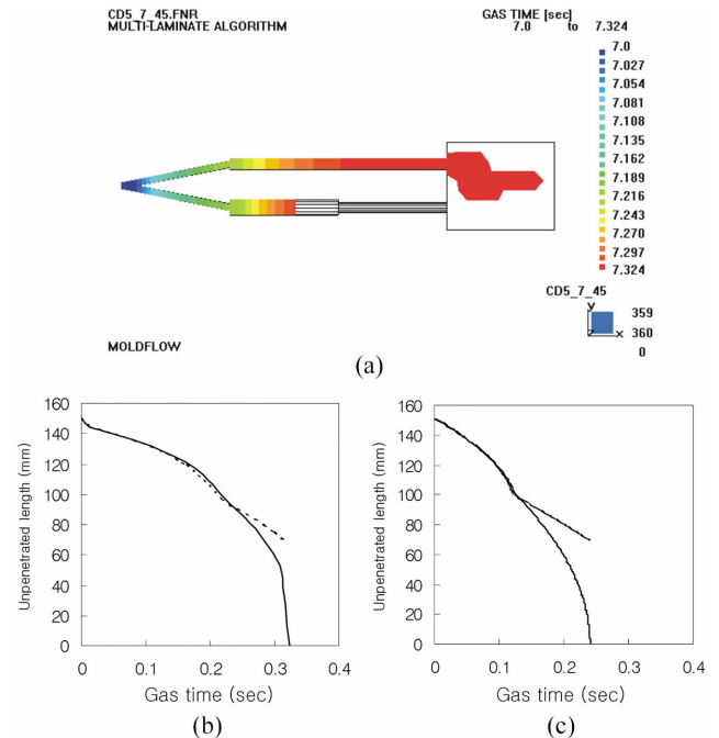
Fig. 17. (a) The geometry is similar to Fig. 8 except that diameter of pipe 21 is 7 mm. Instead of a thick cavity of two square plates, branching runners with diameter of 3 mm are attached at the left hand side to deliver resin to pipes at both upper side and lower side; (b) Time evolution of gas penetration length from Fig. 17(a); (c) Model prediction (solid line: upper side, dotted line: lower side).
