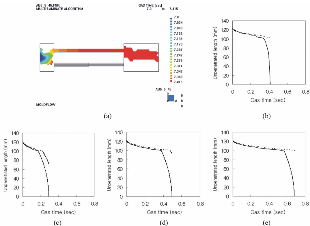
Fig. 8. (a) Pipe 11 with a diameter of 5 mm and a length of 50 mm is connected to pipe 12 with a diameter of 5 mm and a length of 50 mm. Pipe 21 with a diameter of 5 mm and a length of 50 mm is connected in series with pipe 22 with a diameter of 4.5 mm and a length of 50 mm; (b) Time evolution of gas penetration length from Fig. 8(a); Model predictions; (c) \hat{\theta}=0.93 ; (d) \hat{\theta}=2/3\pi ; (e) \hat{\theta}=\pi (solid line: upper side, dotted line: lower side).
