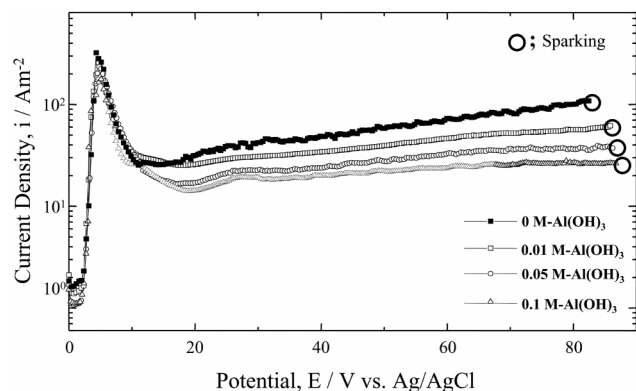
Fig. 1. The current density/potential profiles at a scan rate of 60 mV/s in 1 M NaOH containing various \text{Al(OH)}_3 concentrations at 298 K.
