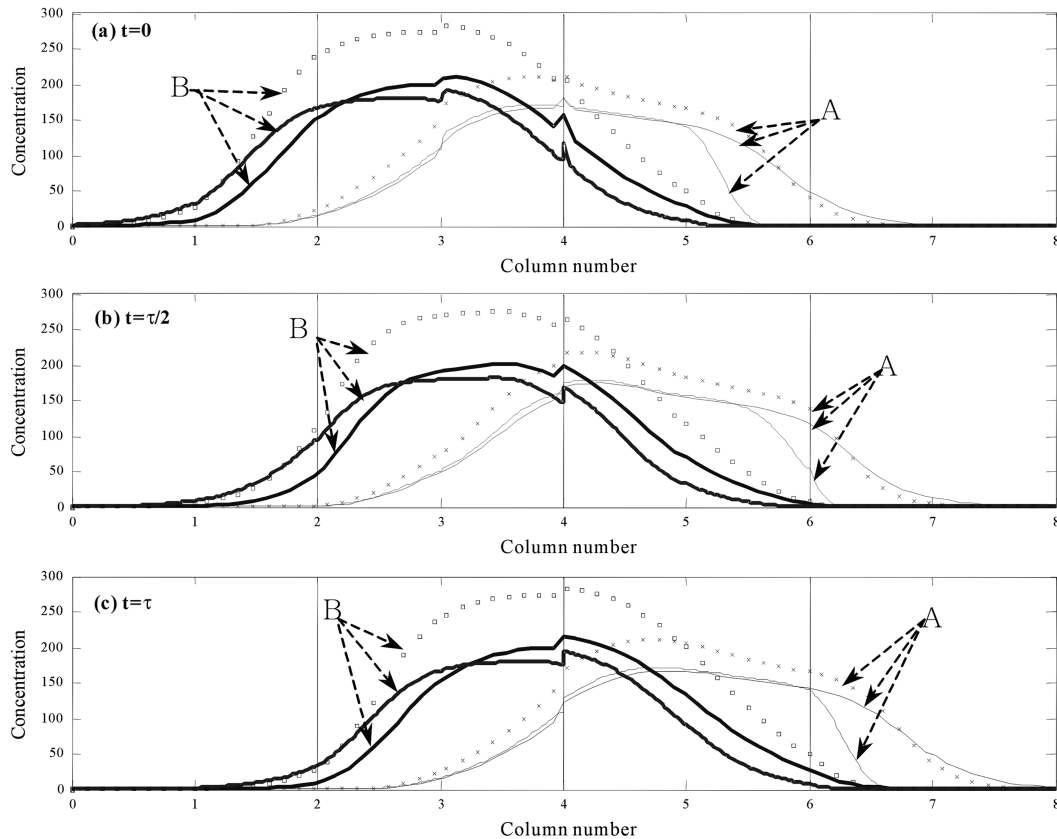
Fig. 5. Comparison of SMB simulation results for the level 2 (solid lines), level 3 repeated (dashed lines) and the reference case (points) at three different moments of the cycle time ( N_{\text{shift}}=44 ).
