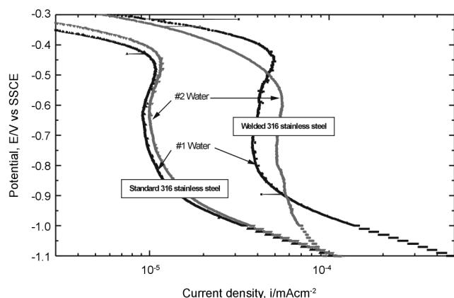
Fig. 11. Cathodic polarization curves of welded STS 316 and standard STS 316 in #1, #2 water.
