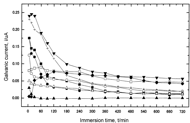
Fig. 2. Galvanic current between welding part STS 316 and STS 304, STS 329, STS 444 in #1 water at 50 °C [Area Ratio (1 : 1); STS 329 (■), STS 444 (●), STS 304 (▲), Area Ratio (1 : 5); STS 329 (□), STS 444 (○), STS 304 (△), Area Ratio (1 : 10); STS 329 (▼), STS 444 (◆), STS 304 (+)].
