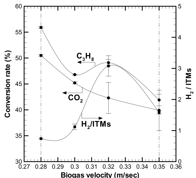
(b) Biogas conversion rate and H 2 /Intermediates ratio
