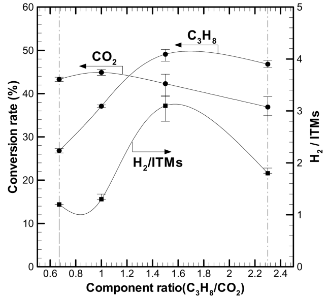
(a) Biogas conversion rate and H 2 /Intermediates ratio
