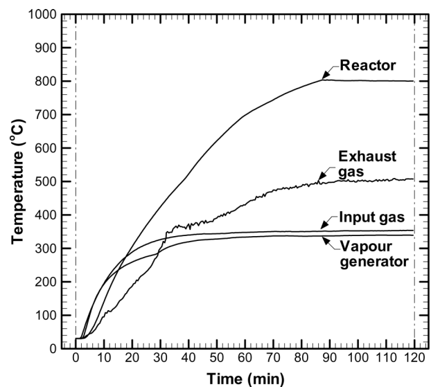
Fig. 2. Initial operating characteristic of the reformer.
