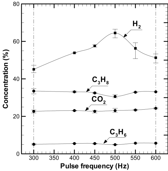
(a) Concentration of selected SynGas
