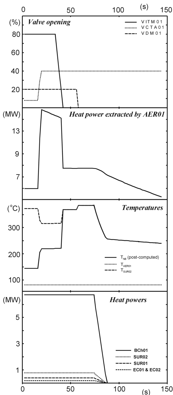
Fig. 6. Variation of operating parameters and consequent reply of the model (b).
