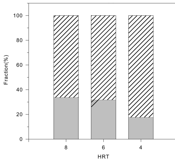
(a) aerobic 1
