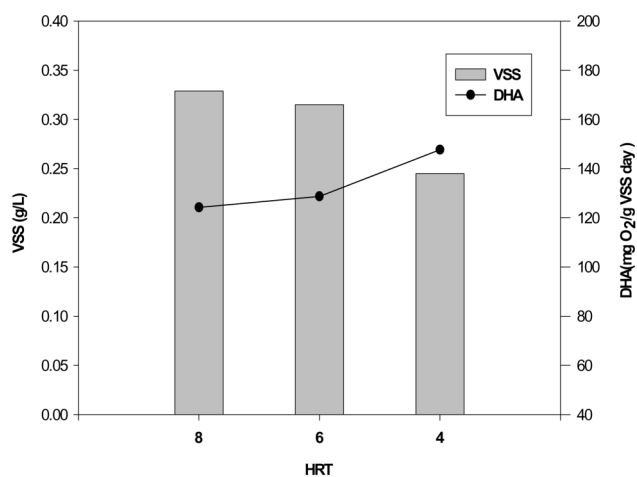
(a) aerobic 1
