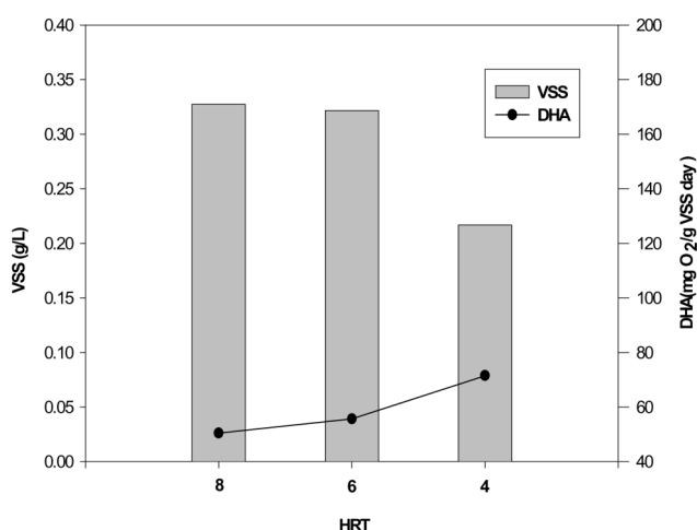
(b) aerobic 2
