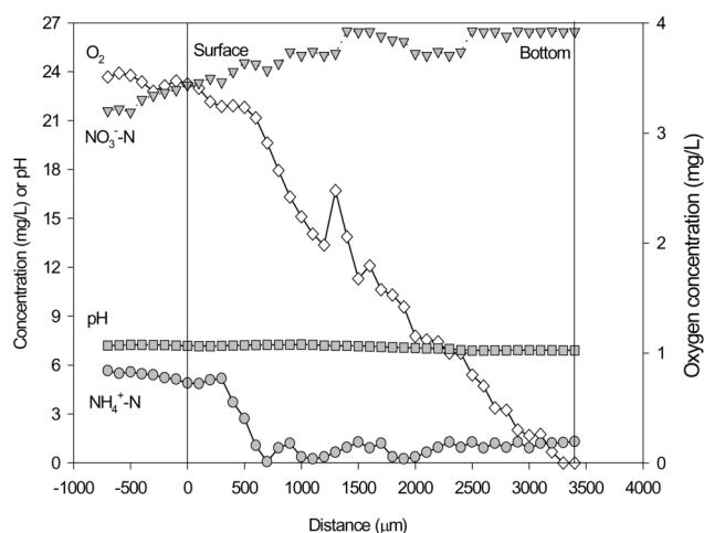
(a) aerobic 1
