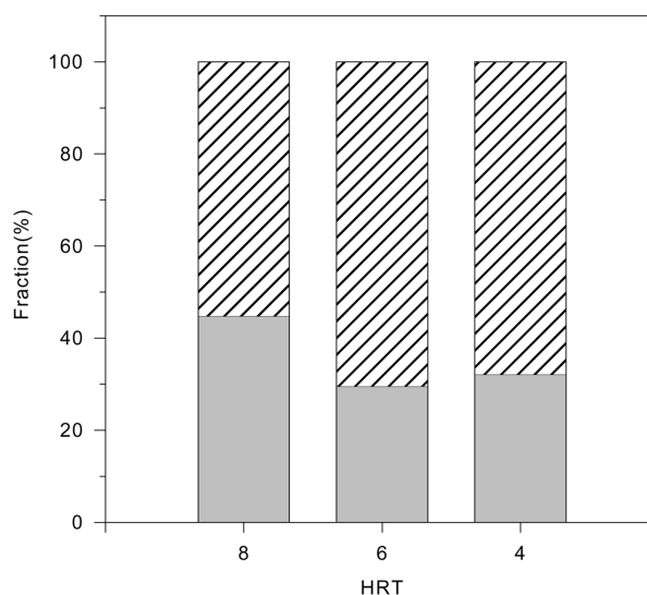
(a) aerobic 1
