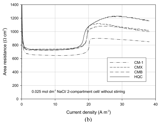
Fig. 4. Current-resistance (I-R) curves of cation-exchange membranes. (a) S-PES membranes; (b) Commercial membranes
