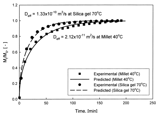
Fig. 7. Typical curve on the ratio of the total amount of the evaporated moisture, M_t/M_0 as a function of the time elapsed with the predicted value of Eq. (8).
