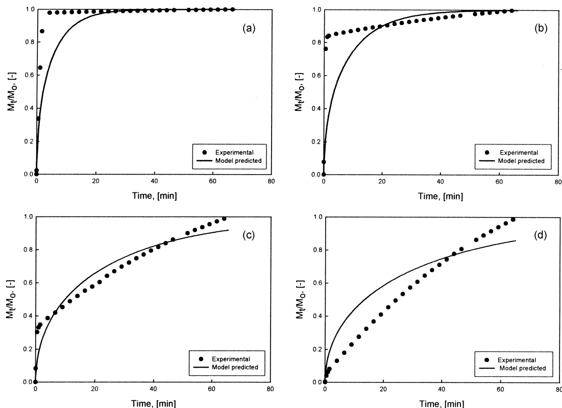
Fig. 8. Four time trials tested to optimize the effective diffusion coefficient of PVC particles at 70^\circ\text{C} .
