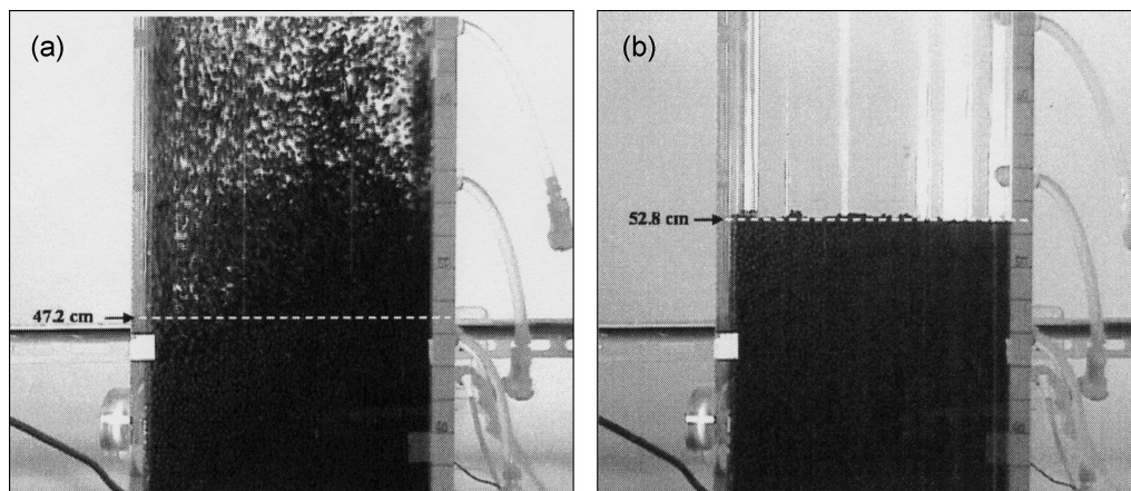
Fig. 3. Typical snapshots for determining the dense bed height after shutting-off of the gas supply: (a) snapshot at t=2.47 s after shutting-off of the gas supply, (b) snapshot at t=20 s after shutting-off the gas supply.
