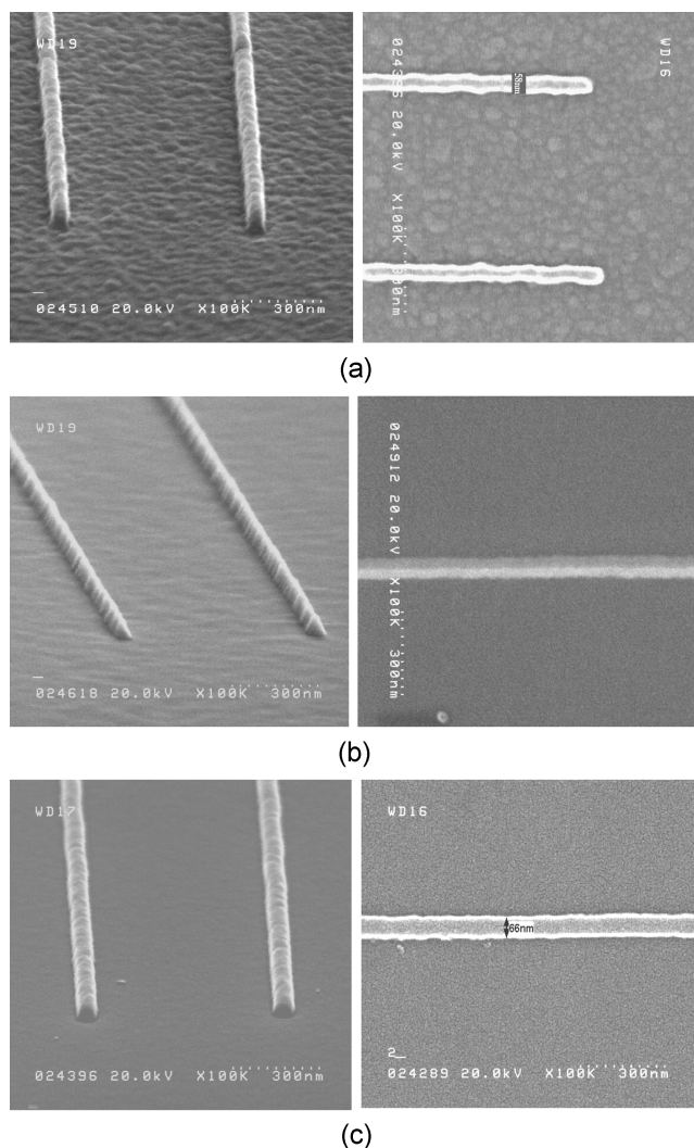
Fig. 4. FESEM micrographs of the polysilicon thin films etched by (b) Cl 2 /Ar and (c) HBr/Ar gases. The resist profile before etching is shown in (a).
