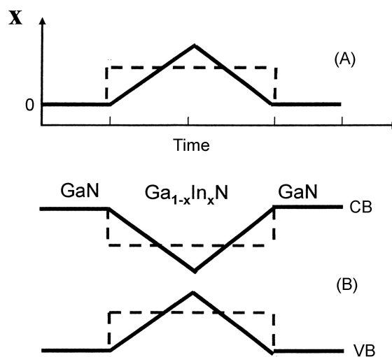
Fig. 1. (A) Variation of In content (x) with time during the growth of InGaIn well layer and (B) energy structure of a triangular quantum well (solid line) compared with rectangular one (dotted line).
