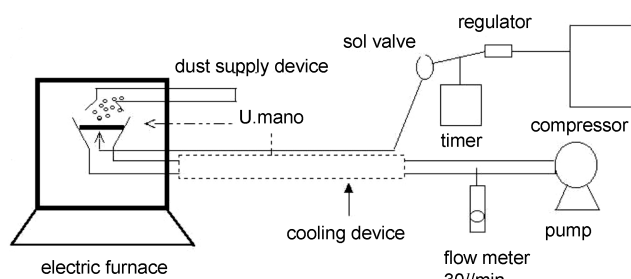
Fig. 2. Schematic of the experimental set up.
