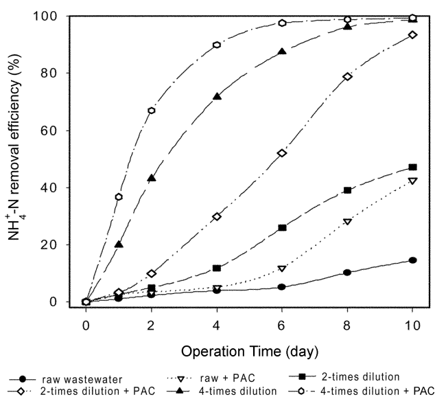
Fig. 12. \text{NH}_4^+\text{-N} removal efficiencies with respect to dilution ratios and PAC addition.
