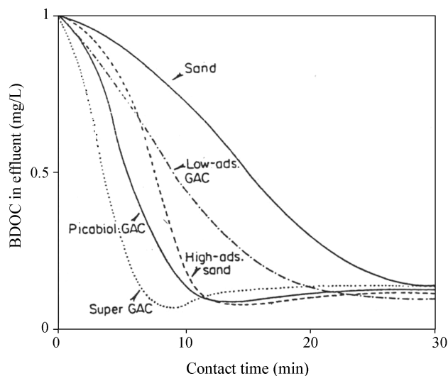
Fig. 3. Effect of types of filter media on the performance of biofilter [Billen et al., 1992].
