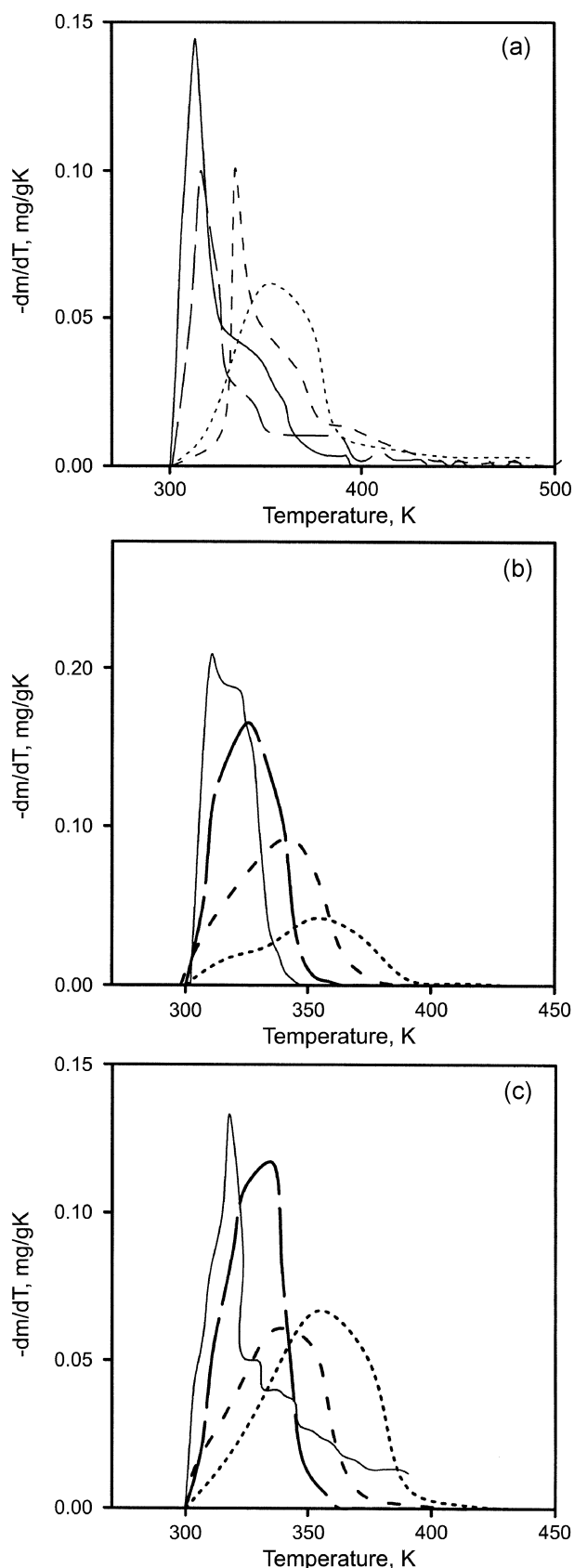
Fig. 6. TPD profiles of (a) TCE, (b) PCE and (c) \text{CCl}_4 from RH-MCM-41 at various heating rates. — 3 K \text{min}^{-1} , — 5 K \text{min}^{-1} , - - - 12 K \text{min}^{-1} , ..... 20 K \text{min}^{-1}
