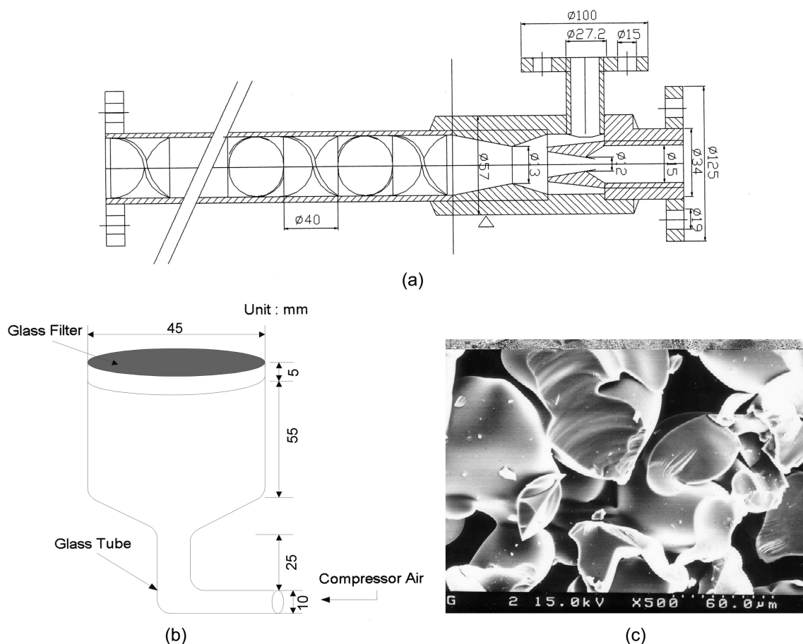
Fig. 2. Schematic diagram of bubble generators in this study.
