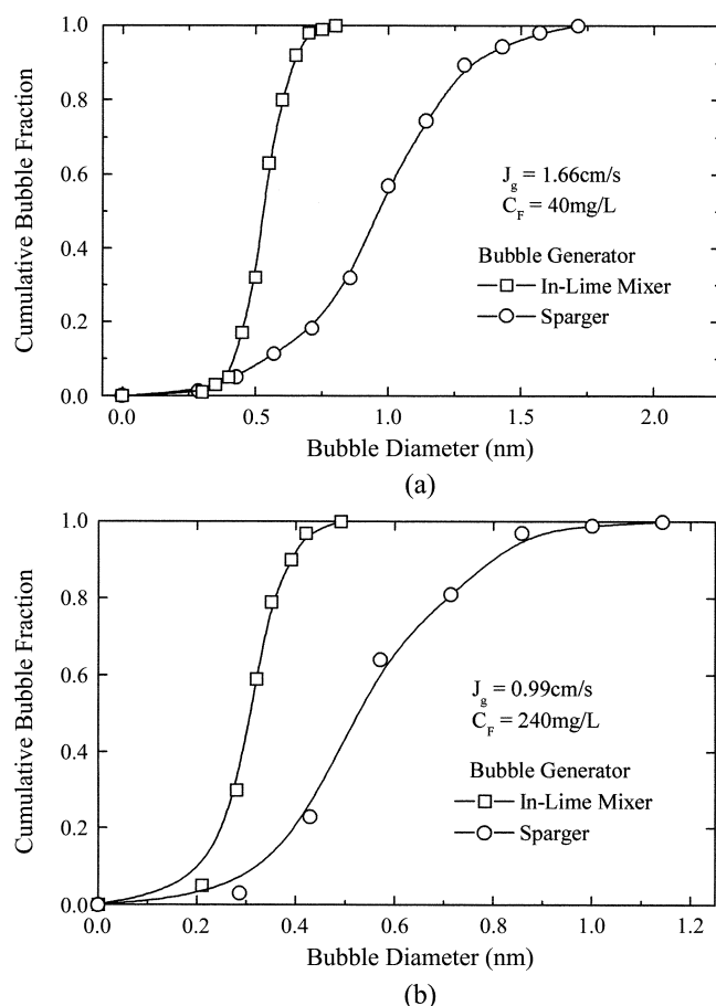
Fig. 6. Comparison with cumulative fraction of bubble formed by in-line mixer and sparger bubble-generator under the different operating condition: (a) C_F = 40 \text{ mg/L} and J_g = 1.66 \text{ cm/s} , (b) C_F = 240 \text{ mg/L} and J_g = 0.99 \text{ cm/s} .
