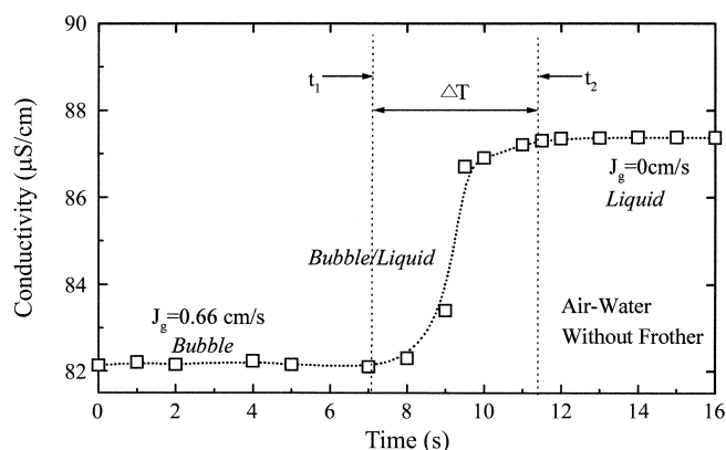
Fig. 3. Relation with conductivity and bubble behavior time in the flotation cell.
