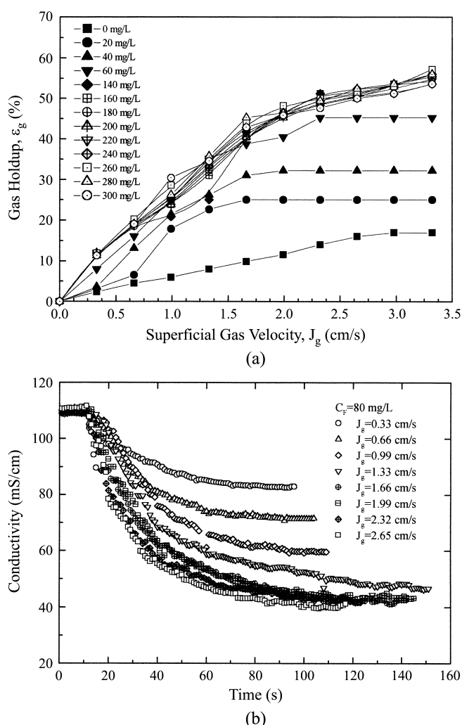
Fig. 7. Gas holdup of bubble formed by in-line mixer bubble-generator: (a) the measurement by the water manometer; (b) by the conductivity meter.
