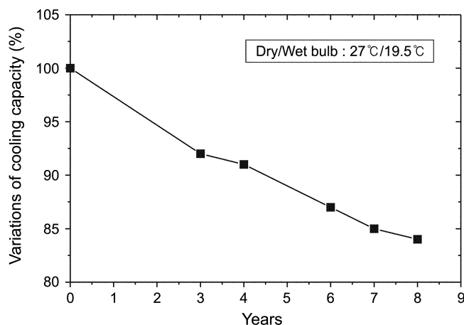
Fig. 7. Chronological variations for cooling capacity of evaporator heat exchangers in air-conditioners used in the seaside inn at the same pressure drop of initial heat exchangers.
