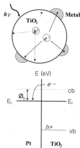
Fig. 10. Model diagram for a Pt-TiO 2 that shows the flow of cb electrons from the TiO 2 to Pt ( \Phi_s ; Schottky barrier).
