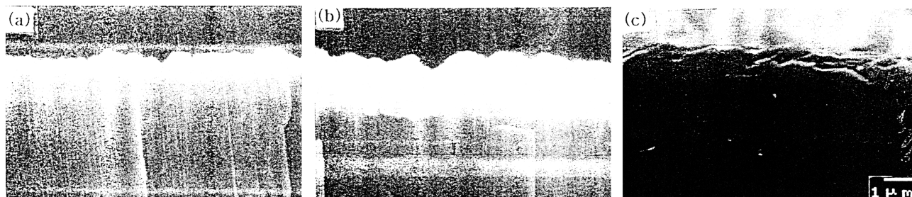
Fig. 4. The cross sectional SEM image of the film grown at 815 °C for (a) 10 min, (b) 20 min and (c) 30 min with O 2 partial pressure of 3.2 Torr and preheating zone temperature of 380 °C.
