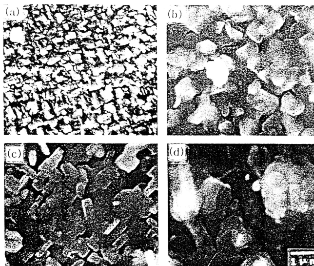
Fig. 2. Scanning electron microscopic images of the films grown at (a) 760 °C, (b) 800 °C, (c) 815 °C and (d) 860 °C for 20 min with O_2 partial pressure of 3.2 Torr and preheating zone temperature of 380 °C.
