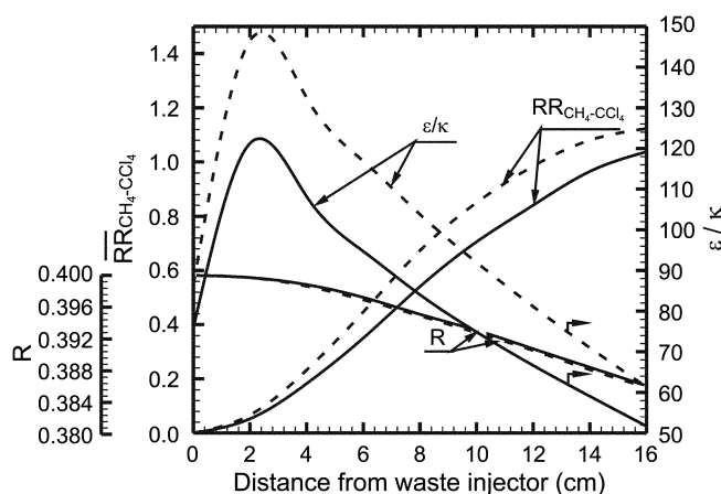
Fig. 8. Selected predictions for Flame 2, with V_w changed to 5 m/s.
