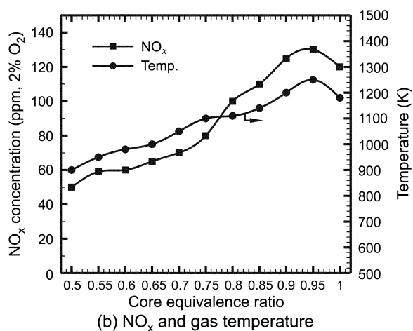
Fig. 9. DREs, selected species measurements and temperature as a function of core equivalence ratio at auxiliary burner.
