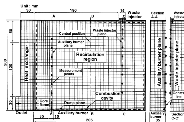
Fig. 2. Computational grid with measurement points and physical dimensions.
