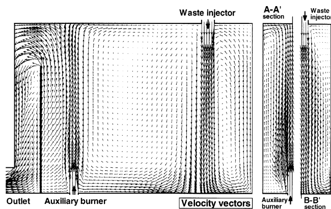
Fig. 4. Calculated velocity vector fields.
