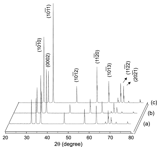
Fig. 4. Typical X-ray diffraction patterns of GaN and Mg-doped GaN micro-crystals; (a) sample A and (b) sample B, (c) sample C (Mg=0.34 wt%). The growth was carried out at 1,000^\circ\text{C} and 1 atm with 50 sccm \text{NH}_3 .
