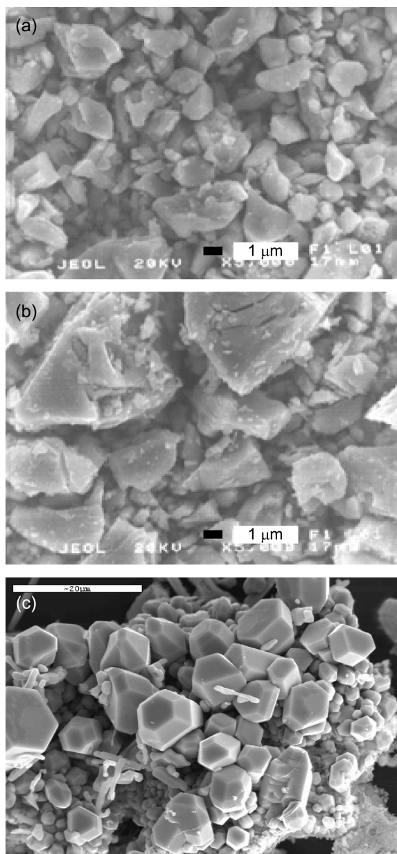
Fig. 3. SEM images for GaN and Mg-doped GaN micro-crystals; (a) sample A and (b) sample B, (c) sample C (Mg=0.34 wt%). The growth was carried out at 1,000^\circ\text{C} and 1 atm with 50 sccm \text{NH}_3 .
