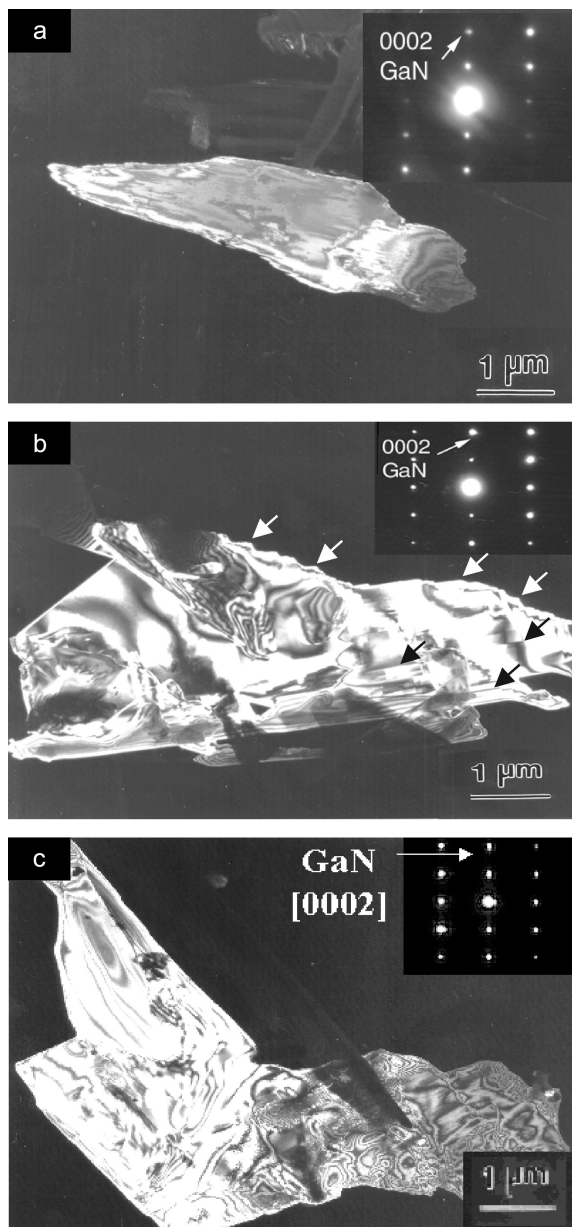
Fig. 5. The dark-field micrographs and the corresponding selected area diffraction pattern (SADP) along the electron beam direction B=[01\bar{1}0] with the reflection vectors g=0002 ; (a) sample A and (b) sample B, (c) sample C (Mg=0.34 wt%). The growth was carried out at 1,000 °C and 1 atm with 50 sccm NH_3 .
