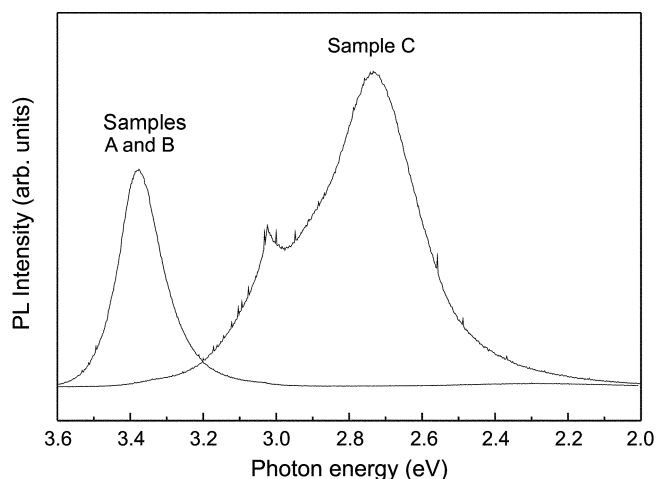
Fig. 6. Photoluminescence spectrums for samples A, B, and C (Mg =0.34 wt%) at room temperature. The growth was carried out at 1,000 °C and 1 atm with 50 sccm NH_3 .
