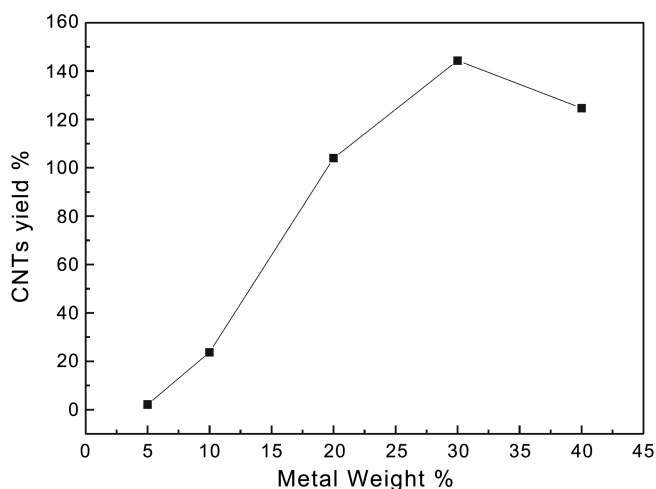
Fig. 3. Variation of deposited carbon yield with metal wt% in the catalysts, CNTs grown for 30 min at 800 °C with C_2H_2/H_2 = 10/100 sccm.
