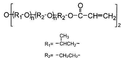
Scheme 1. The molecular structure of tri-block diol diacrylate, t-BDDA.
