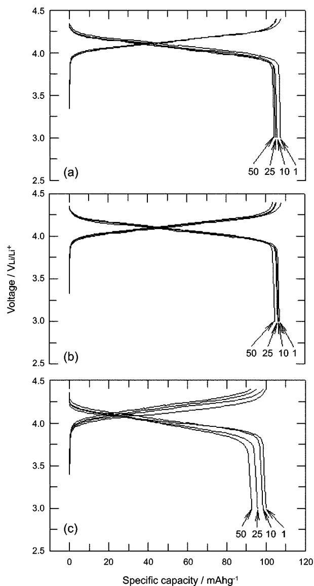
Fig. 3. Charge-discharge curves for \text{Li}/\text{LiAl}_{0.18}\text{Mn}_{1.82}\text{O}_{3.97}\text{S}_{0.03} cells at (a) 25, (b) 50, and (c) 80\text{ }^{\circ}\text{C} as a function of cycle number.
