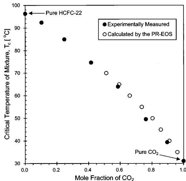
Fig. 5. Critical temperatures of CO 2 /HCFC-22 mixtures as a function of CO 2 composition: a comparison of the experimental and the PR-EOS correlated values.
