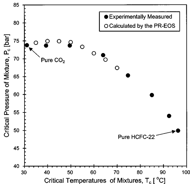
Fig. 4. Critical pressure and temperature of CO 2 /HCFC-22 mixtures: a comparison of the experimental and the PR-EOS correlated values.
