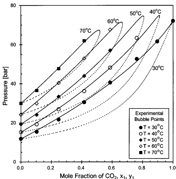
Fig. 3. P-xy diagram at different temperatures for CO 2 (1)/HCFC-22(2) system. The symbols are experimental bubble points, and the solid and dashed lines are the bubble point and dew point curves correlated by the PR-EOS, respectively ( k_{ij} = -0.0024 at 30 °C, -0.0108 at 40 °C, -0.0167 at 50 °C, -0.0047 at 60 °C, -0.0045 at 70 °C).
