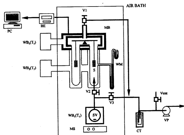
Fig. 1. Schematic diagram of vapor sorption apparatus
