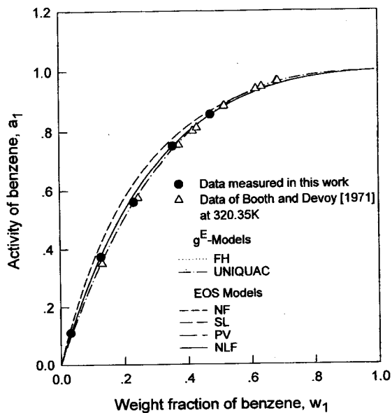
Fig. 7. Measured and calculated activities of benzene in PPO ( M_n :2,000) at 298.15 K.
