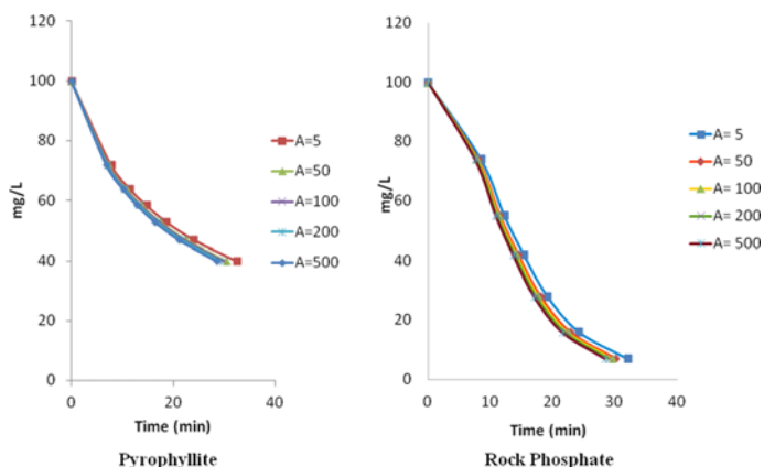
Lead adsorption on low cost mineral adsorbents at an initial lead concentration of 100 mg/L for different values of A, ranging from 5 to 500 ((L/mg)).
