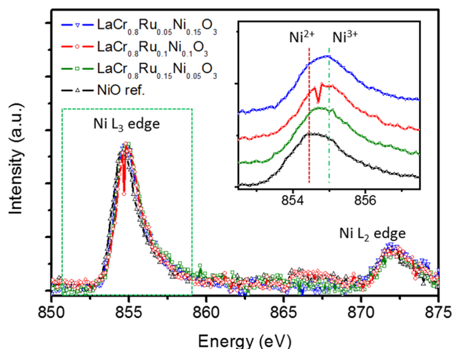
Fig. 4. The normalized XANES spectra of Ni \text{L}_{3,2} -edge of the \text{LaCr}_{1-(x+y)}\text{Ru}_x\text{Ni}_y\text{O}_3 perovskite micro-tubulars: ( x=0.15 , y=0.05 ), ( x=0.1 , y=0.1 ) and ( x=0.05 , y=0.15 ), with inset for the magnified XANES spectra.
