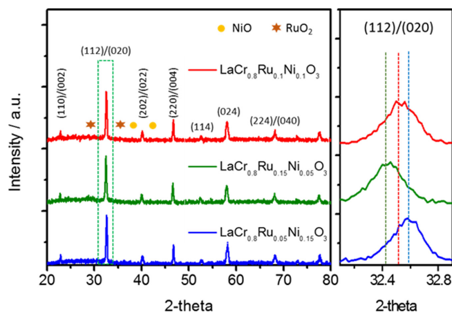
Fig. 3. XRD patterns and evolution of phases of the \text{LaCr}_{1-(x+y)}\text{Ru}_x\text{Ni}_y\text{O}_3 perovskite micro-tubulars: ( x=0.15 , y=0.05 ), ( x=0.1 , y=0.1 ) and ( x=0.05 , y=0.15 ), with inset for the magnified XRD patterns.
