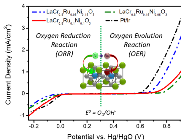
Fig. 7. ORR and OER polarization curves of the micro-tubular \text{LaCr}_{1-(x+y)}\text{Ru}_x\text{Ni}_y\text{O}_3 perovskite: ( x=0.15, y=0.05 ), ( x=0.1, y=0.1 ) and ( x=0.05, y=0.15 ), at the measurement condition of -0.25 to 0.95 V vs. Hg/HgO with the scan rate of 5 mV/s and RDE rotation speed of 1600 rpm in the \text{O}_2 -saturated 6 mol KOH.
