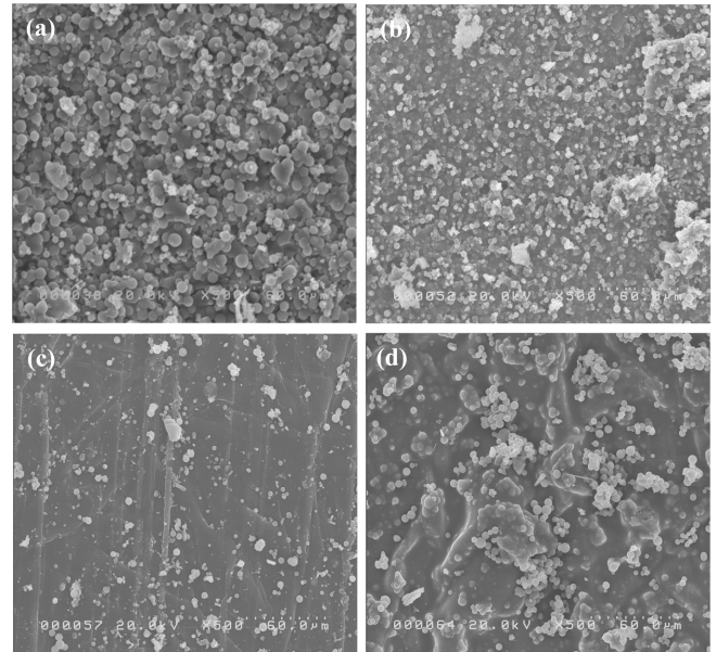
Fig. 6. SEM images of phenol resin after treated with various supercritical solvents; (a) methanol 380 °C, 223 bar (mean particle size 2.84 \mu\text{m} ) (b) ethanol, 380 °C, 177 bar (mean particle size 2.12 \mu\text{m} ) (c) acetone, 380 °C, 125 bar (mean particle size 1.95 \mu\text{m} ) (d) water, 380 °C, 219 bar (mean particle size 2.47 \mu\text{m} ).
