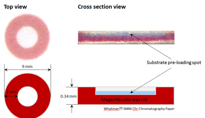
Fig. 1. Schematic of the paper-based neuraminidase assay sensor (PNAS). The PNAS sensor was simply designed as reservoir type. It was patterned with circular hydrophilic zone ( d \sim 5 mm) surrounded by a hydrophobic magenta color wax barrier.
