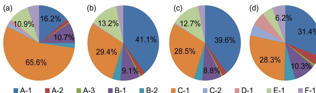
Fig. 6. Patent distribution of technology groups for lubricants production. (a) USA; (b) Japan; (c) EU and; (d) Korea.
