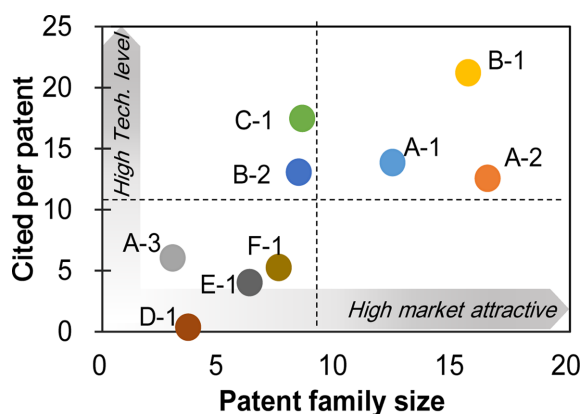
Fig. 5. Relative technical and market positions of major technology groups in lubricants production industries.
