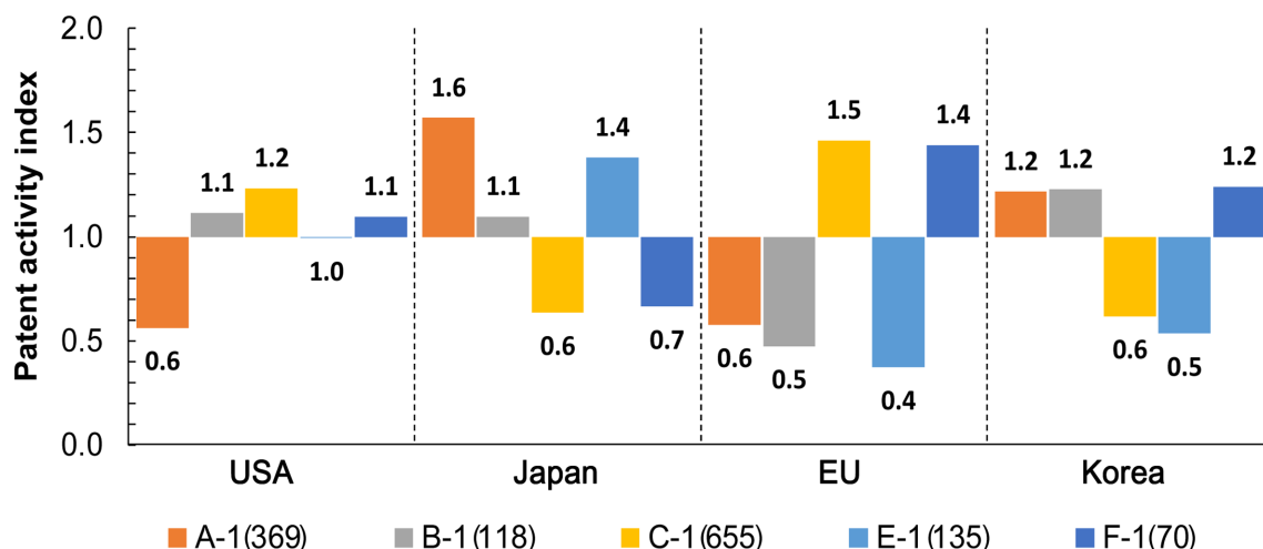
Fig. 7. Patent activity index of major technology groups for lubricants production. The value in parentheses denotes the number of patent applications in a technology group.
