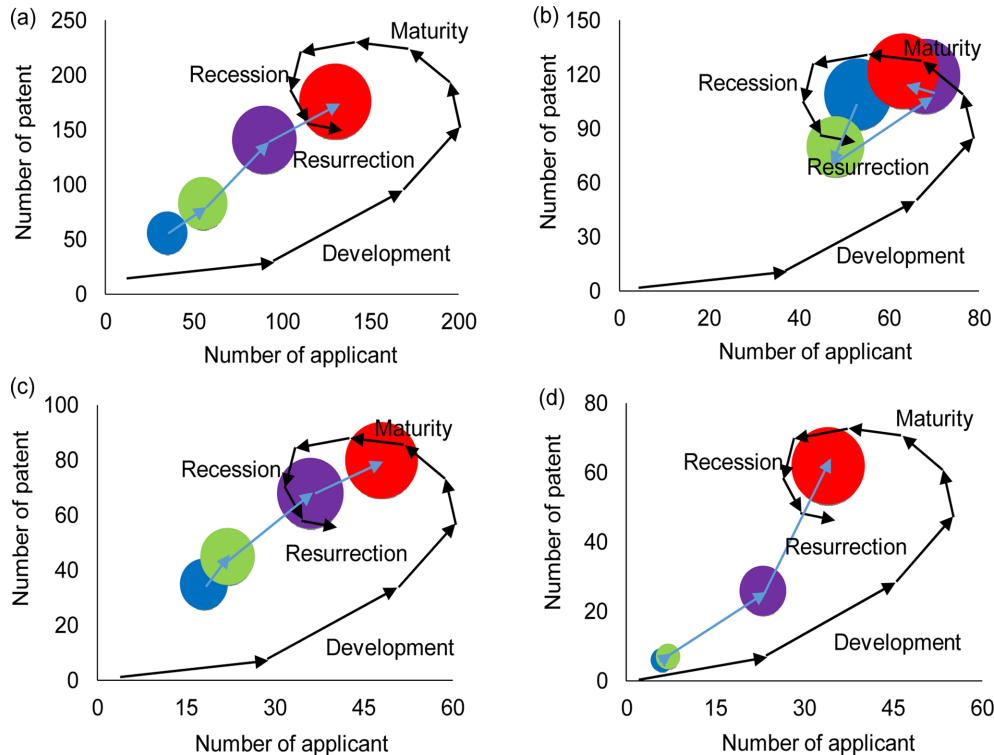
Fig. 3. Patents portfolio analysis of lubricants production technologies of the selected countries on the year of application. (a) USA; (b) Japan; (c) EU and; (d) Korea.
