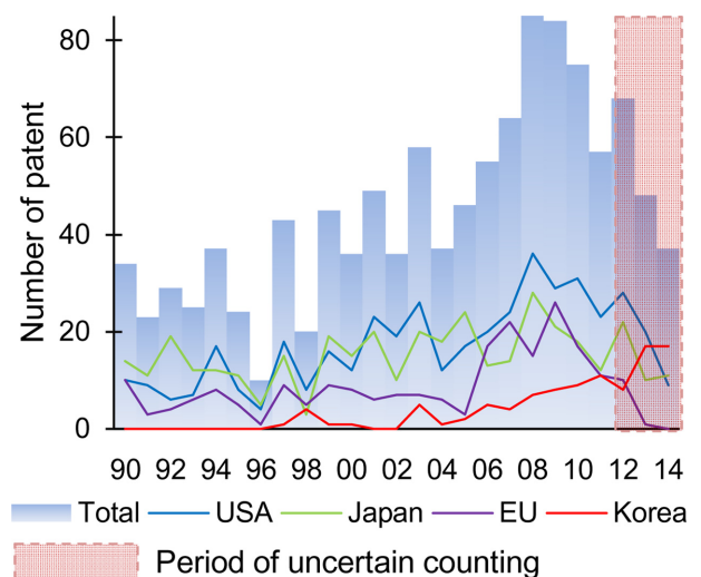
Fig. 2. The annual number of patents of lubricants production technology by country; note that the time period (2012~2014) which is marked with red-colored box represent the number of patent may not be exact due to the presence of unpublished data.
