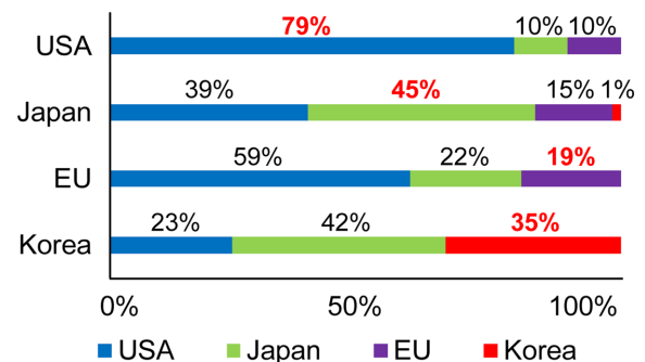
Fig. 4. Distribution of major nationalities of patent holders of the selected countries; red-colored values represent the share of native registration of each country.
