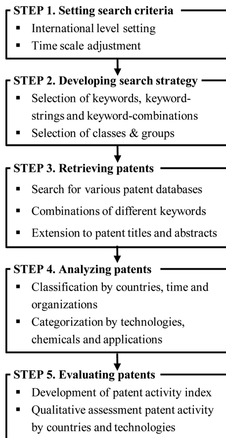
Fig. 1. Main steps for analysis and evaluation of patent activities.
