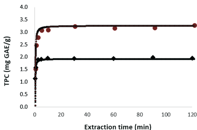
Fig. 5. Simulation of hot-water and hot-water with 40% ethanol using Peleg's model. ●: Experimental data from hot-water extraction with 40% ethanol ◆: Experimental data from hot-water extraction, —: Simulation using Peleg's model.
